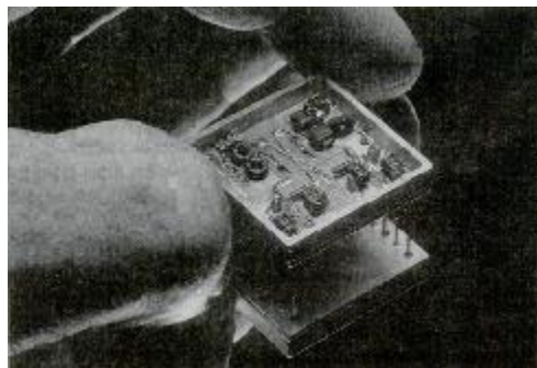
Figure 7: Missile Guidance Beamformer
