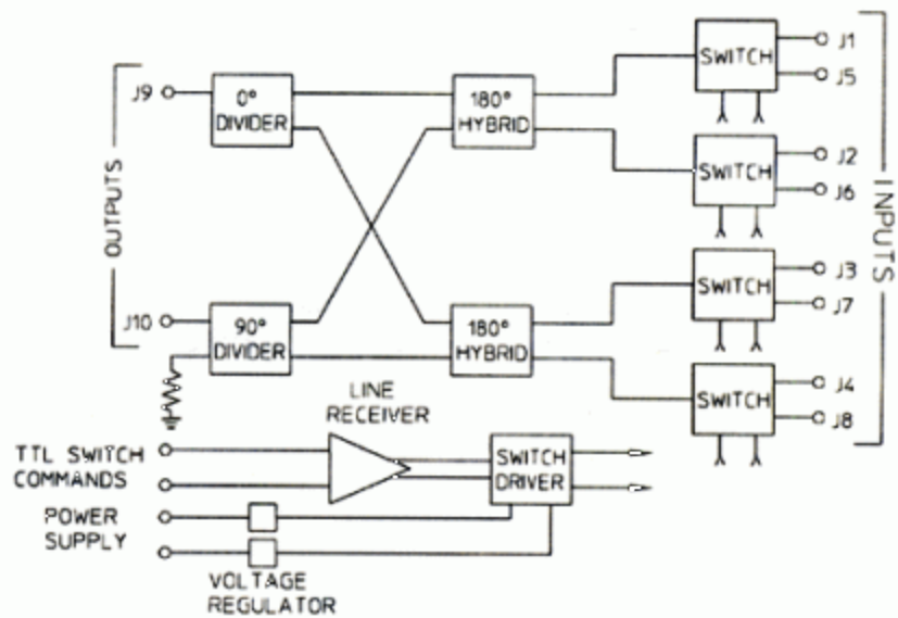
Figure 8: Beamformer Subsystem Schematic
